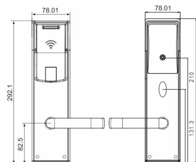
Lock Body Dimension
