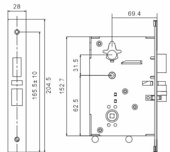
Mortise Body Dimension
