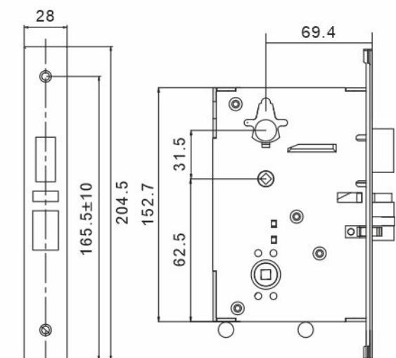
Mortise Body Dimension
