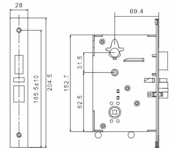
Mortise Body Dimension
