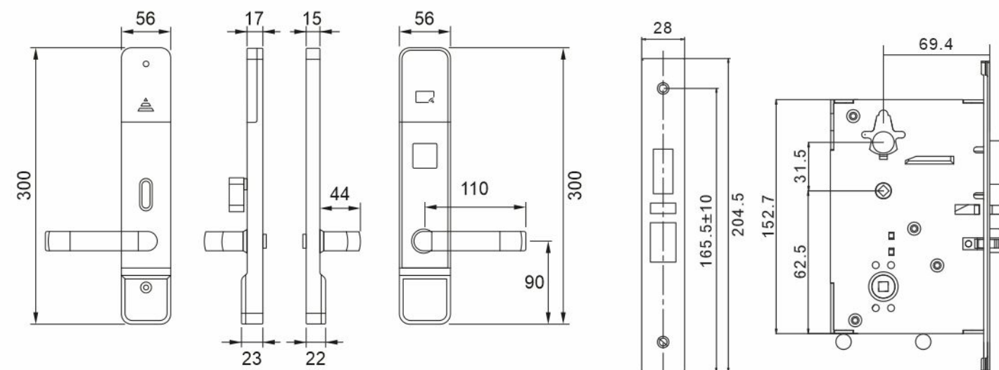
Lock Body Dimension
