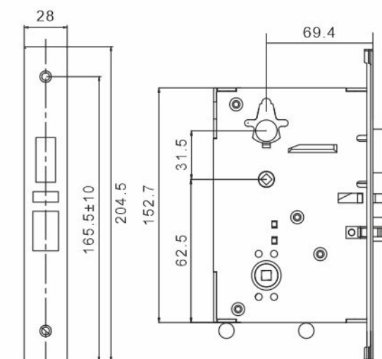
Mortise Body Dimension
