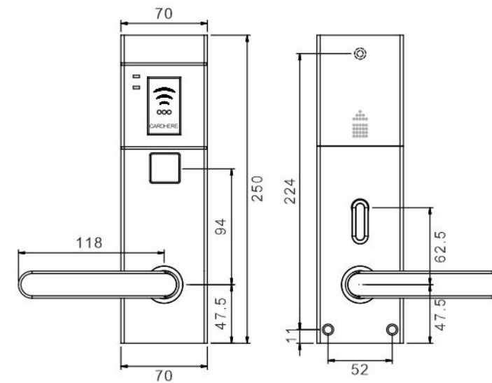
Lock Body Dimension
