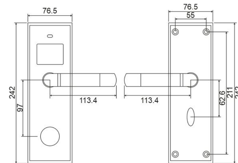
Lock Body Dimension
