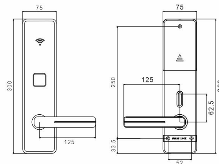
Lock Body Dimension
