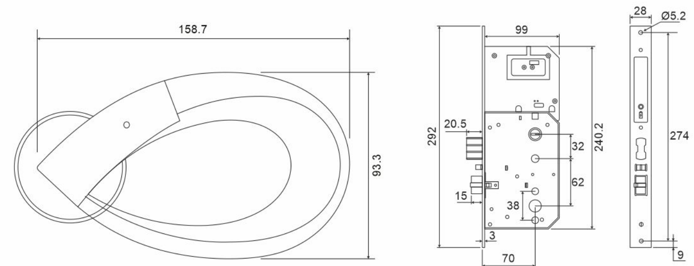
Lock Body Dimension
